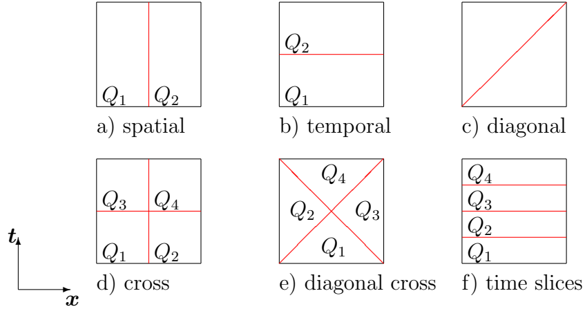
Figure 1: Domain decomposition of the space-time domain Q = \Omega \times (0, T) \subset \mathbb{R}^2 .
